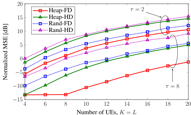
Fig. 11. Normalized MSE versus the number of UEs in CF-mMIMO with \tau \in \{2, 8\} .
