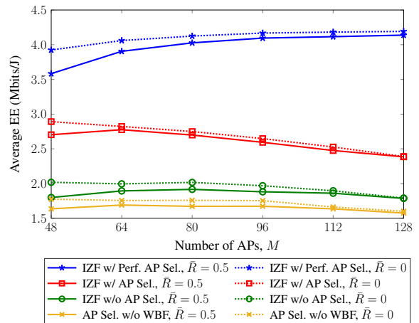
Fig. 10. Average EE versus the number of APs in FD CF-mMIMO under different types of AP selections, with \bar{R} \in \{0, 0.5\} bits/s/Hz.
