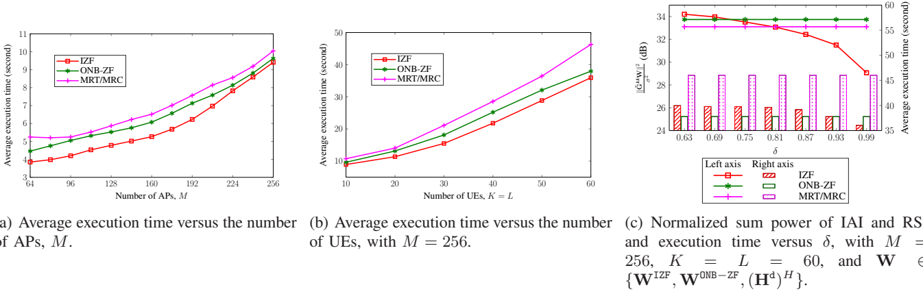
Fig. 14. Average execution time of Algorithm 1 for different transmission strategies in FD CF-mMIMO.
