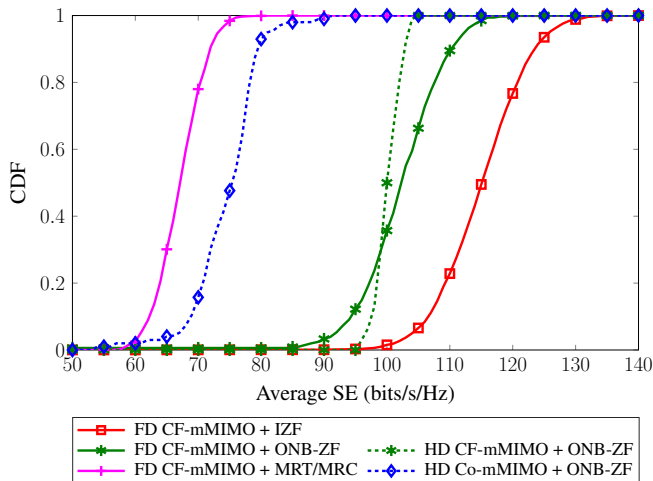
Fig. 5. Cumulative distribution function versus the average SE.
