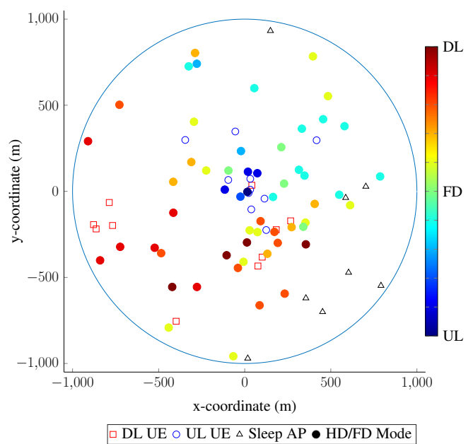
Fig. 8. Operation behavior of APs using the system topology in Fig. 2
