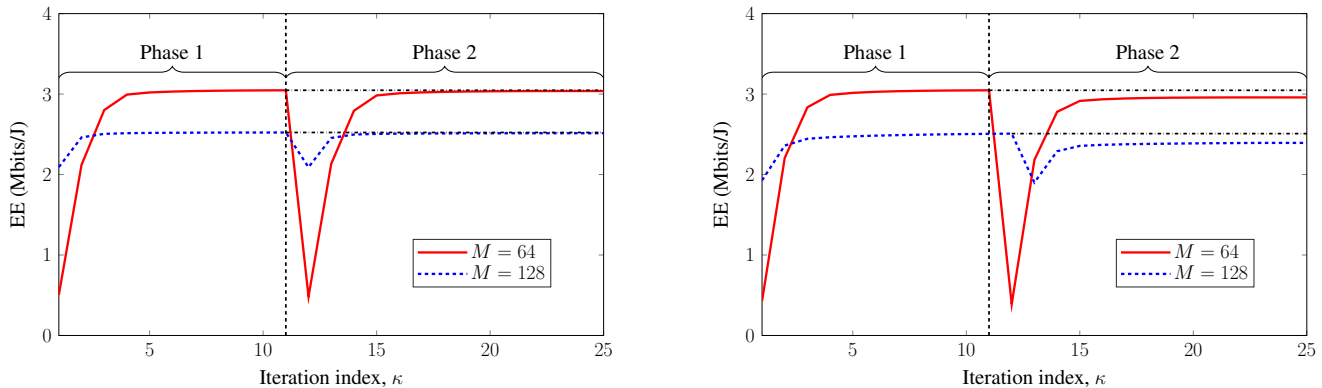
(a) EE convergence behavior of Algorithm 1 in FD CF-mMIMO, with the per-AP power signal ratio \varpi = 0.1\% of 1/M .
